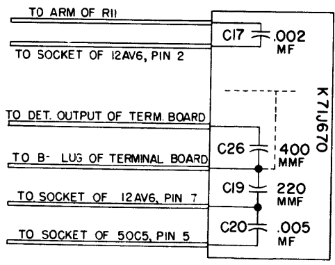
Capacitor RCW-3013
